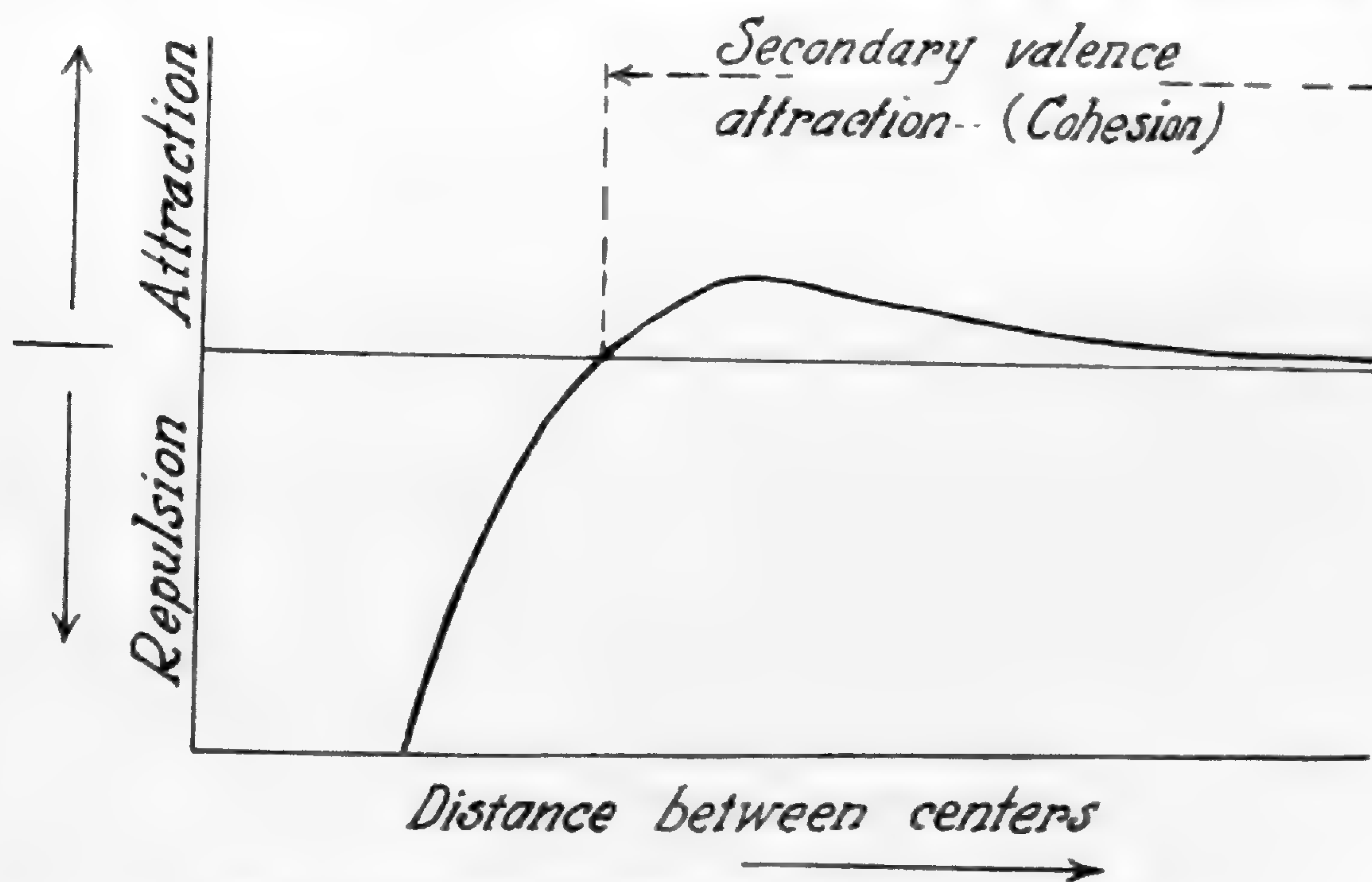
FIG. 5. The attraction between two non-reacting molecules.
